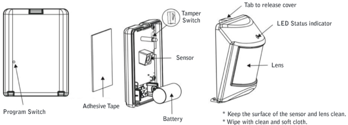
Figure 1: Milan Vortex Wireless Motion Sensor
