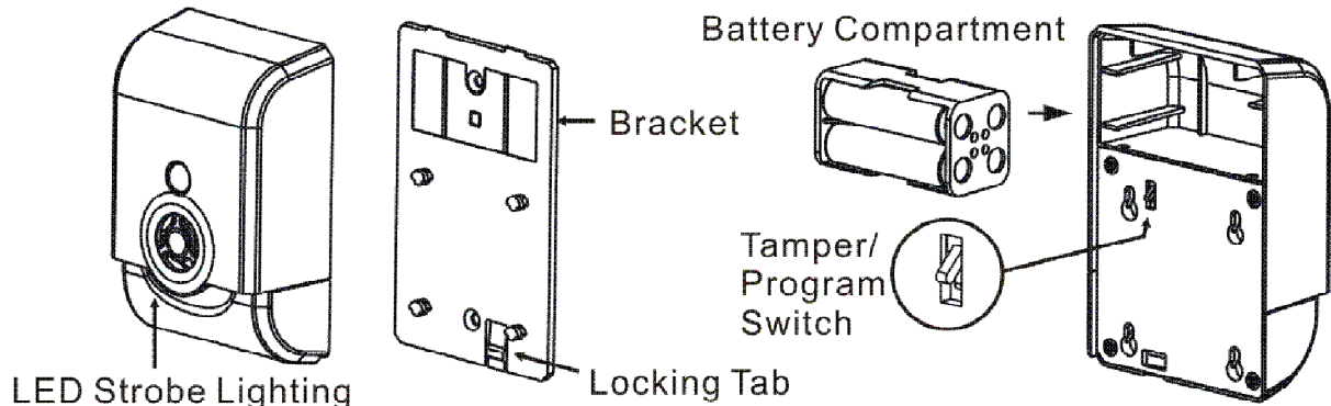
Figure 1: Milan Vortex Wireless Siren
